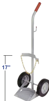
NO. 6108-MRI HEIGHT: 40" DEPTH: 12" WIDTH: 13" WEIGHT: 12 lbs. WHEEL DIA: 8" SOLID RUBBER HOLDS 1 (M or M60) CYL.
